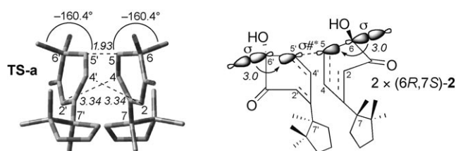
Scheme 4. Structure of TS-a , which leads to (+)-aquatol ( 1a ), with dihedral angles and interatomic distances (Å), and schematic view of “Cieplak–Fallis” interactions (in kcal mol –1 ).
